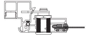
Keyed Lock Security Window Screen Cross Section
