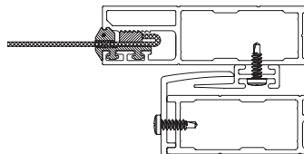
Slimline Security Sliding Screen Door Cross Section
